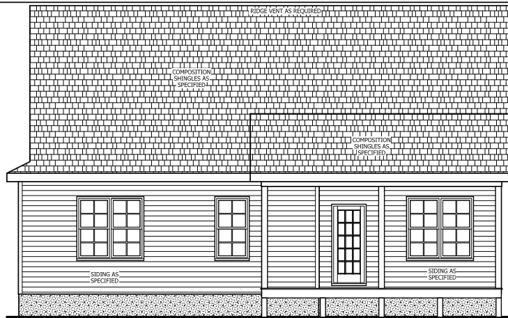
REAR ELEVATION
